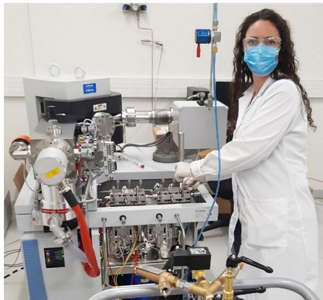
Newly established isotope ratio mass spectrometer facility supporting comparison of CO 2 and CO 2 in air isotope ratio standards, CCQM-P204 and future planned on-demand comparisons BIPM.QM-K3 and BIPM.QM-K4
