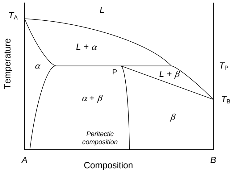
Figure 3. A simple binary peritectic phase diagram.
