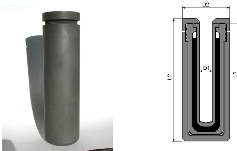
Figure 11. Photograph of a eutectic fixed-point cell and schematic diagram
