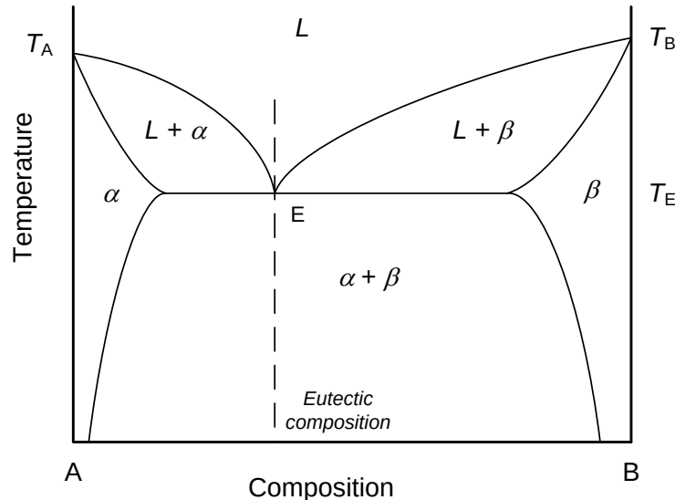
Figure 2. Binary phase diagram for a eutectic.
